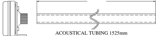
SPEAKER DRIVER
