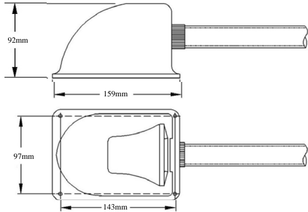
SPEAKER DRIVER
